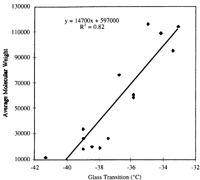
Fig. 1. Aged Estane with a lower M_w has a lower T_g .
