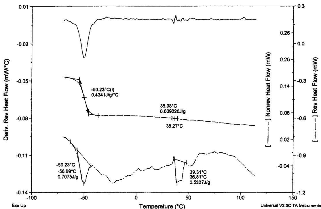
Fig. 3. M-DSC analysis of the binder of PBX 9501 shows the reversible, its derivative, and nonreversible thermal transitions.
