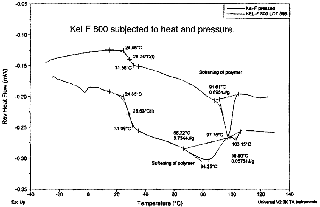
Fig. 5. Hot pressing Kel F 800 affects its thermal properties. Top scan in before and bottom scan is after heating and pressing.
